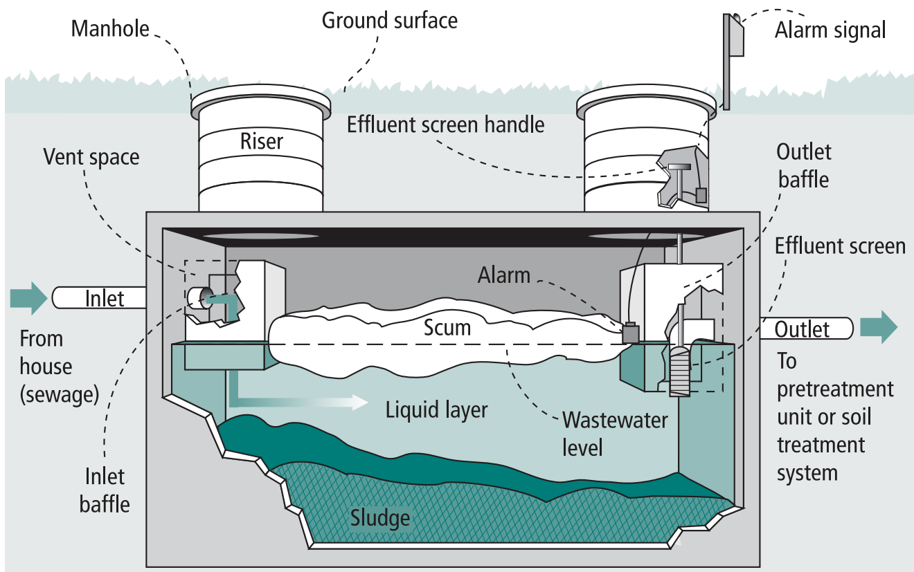
Figure 3 – Septic tank
